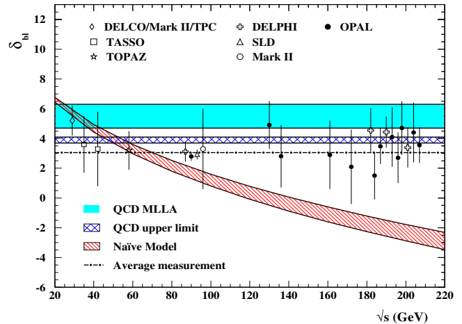
Fig. 1. The difference in the mean charged multiplicities, \delta_{bl} , between heavy and light quark pairs as a function of centre-of-mass energy. The dashed-dotted line is the combined result from all measurements. The MLLA prediction does not include higher-order corrections. See [1] for more details
