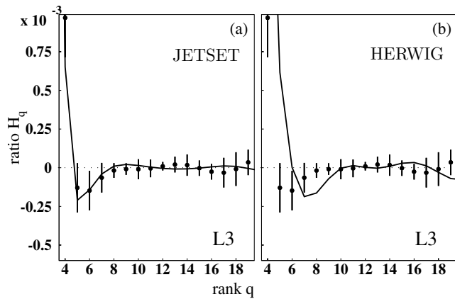
Fig. 2. The H_q moments of the charged-particle multiplicity distributions of L3 compared to the predictions of a JETSET and b HERWIG Monte Carlo models, as reported in [4]
