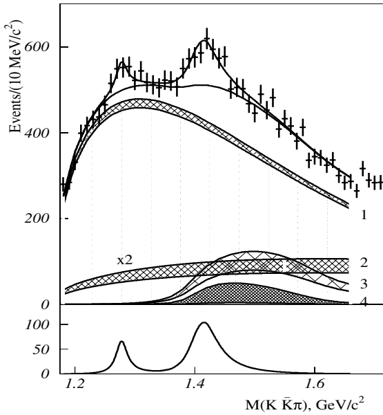
Fig. 4. K_S K^\pm \pi^\mp invariant mass distribution measured by DELPHI [8] with a breakdown into the partial waves for the signals (lower histogram) and the background (one error band). The signals consist of J^{PC} = 1^{++} a_0(980)\pi (first peak) and 1^{++} K^*(892)\bar{K} (second peak). The background includes: (1) isotropic phase space distribution, and (shown magnified by a factor of two) the partial waves of (2) 0^{-+} a_0(980)\pi , (3) 1^{++} K^*(892)\bar{K} , and (4) 1^{++} K^*(892)\bar{K}
