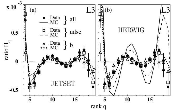
Fig. 3. The H_q moments of the truncated charged-particle multiplicity spectra for all, udsc-, and b-quark events of L3 data compared to the predictions of a JETSET and b HERWIG Monte Carlo models, as reported in [4]
